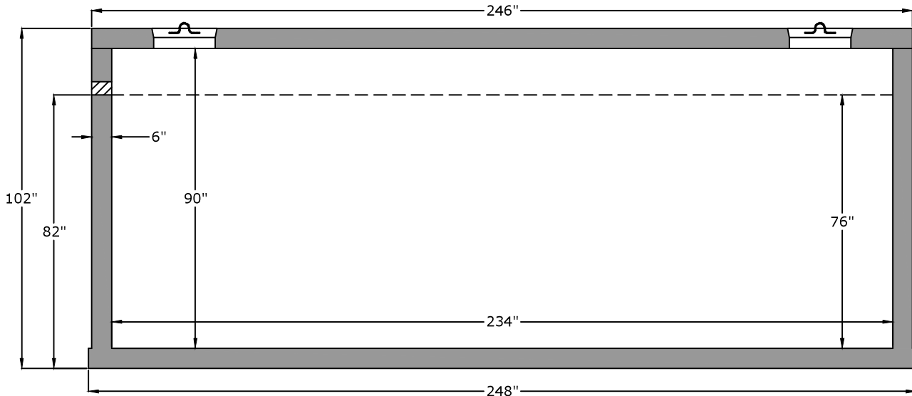
Side View
